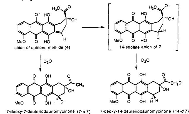
Scheme II. Mechanism Proposed for Deuterium Incorporation in 7-Deoxydaunomycinone from Reduction of Daunomycin in DMSO/D 2 O
