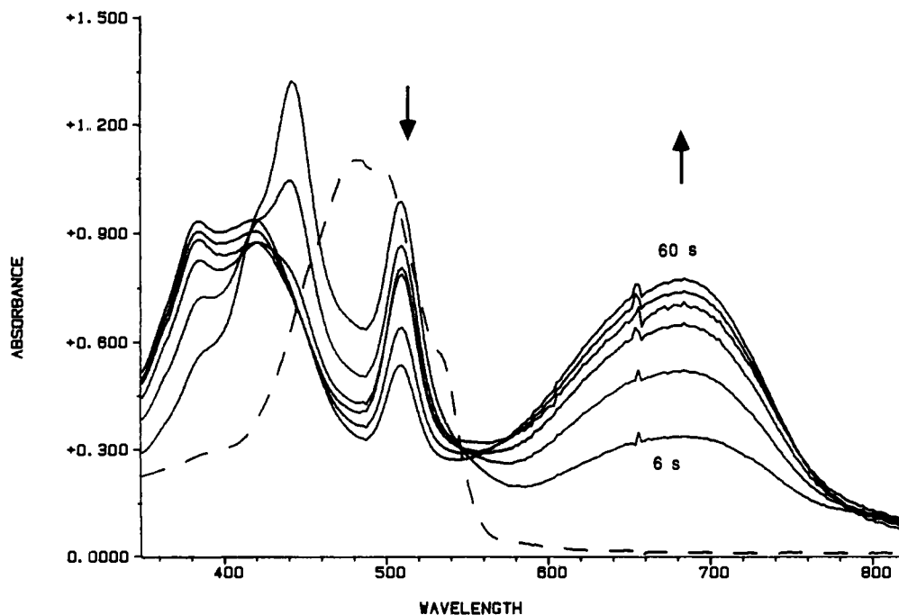
Figure 1. UV-vis spectral changes upon anaerobic reaction of a 9.5 \times 10^{-5} M solution of daunomycin ( 1 ) with 1 mol equiv of dithionite in 5%/95% \text{H}_2\text{O}/\text{DMSO} at 20^\circ\text{C} as a function of time. Spectra were taken at the following times after mixing of the reagents: 6, 9, 15, 30, 45, and 60 s. The spectrum of 1 prior to mixing is shown with dashed lines.
